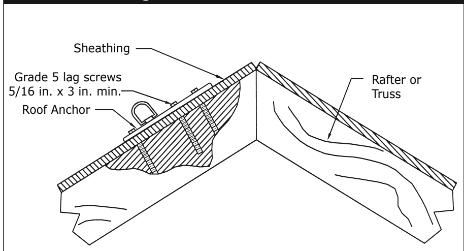
Figure 7 - Anchor Installation
