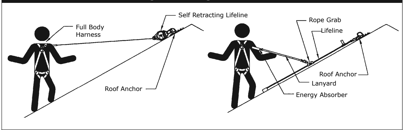
Figure 8 - Making Connections
