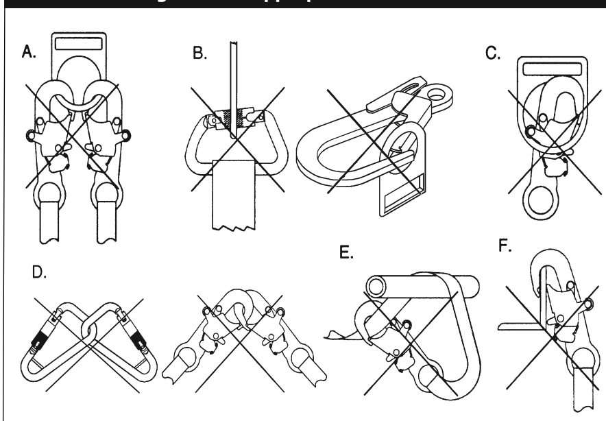
Figure 3 - Inappropriate Connections
