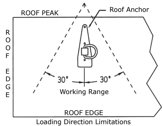
Figure 4 - Swing Fall
